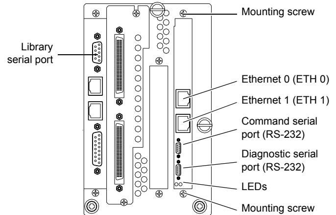
Figure 3 MC300 PMC Ports and Indicators
